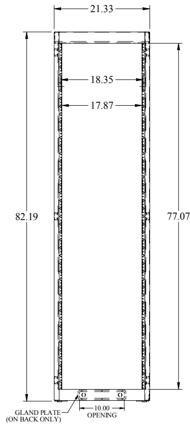
FRONT VIEW
